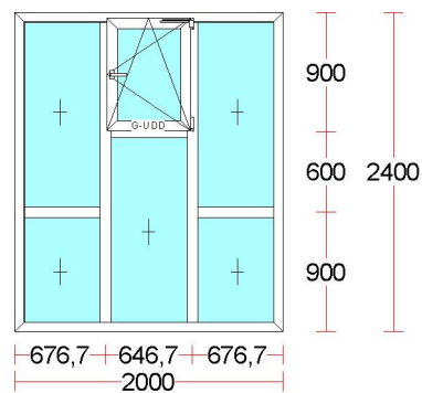
Fereastra08 - 2 buc.
