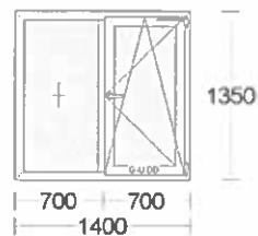
Fereastra02 - 12 buc.
