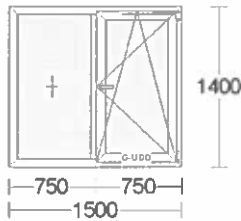
Fereastra06 - 12 buc.
