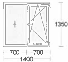
Fereastra02 - 12 buc.
