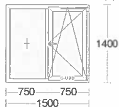
Fereastra06 - 12 buc.
