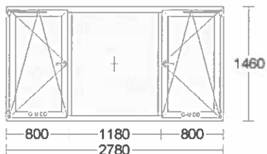
Fereastra01 - 108 buc.
